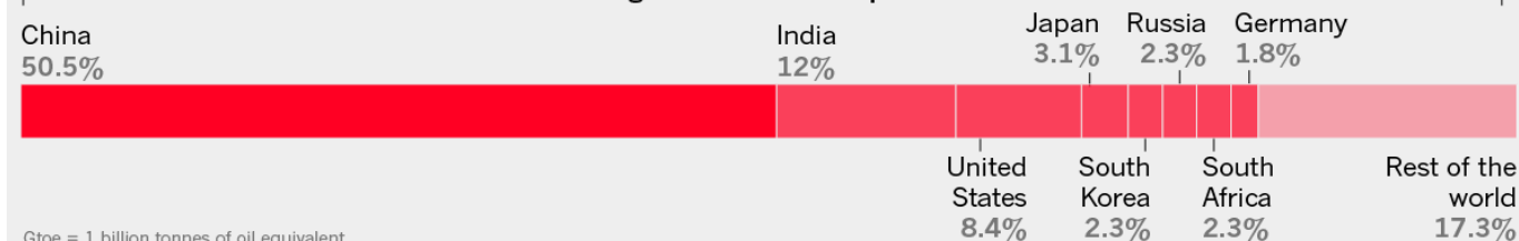
2018 global coal consumption 3.7 Gtoe
