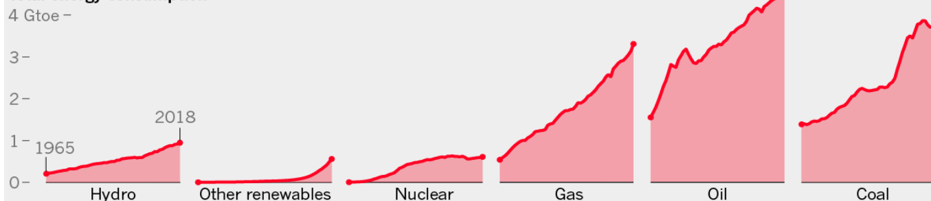
2018 global coal consumption 3.7 Gtoe
